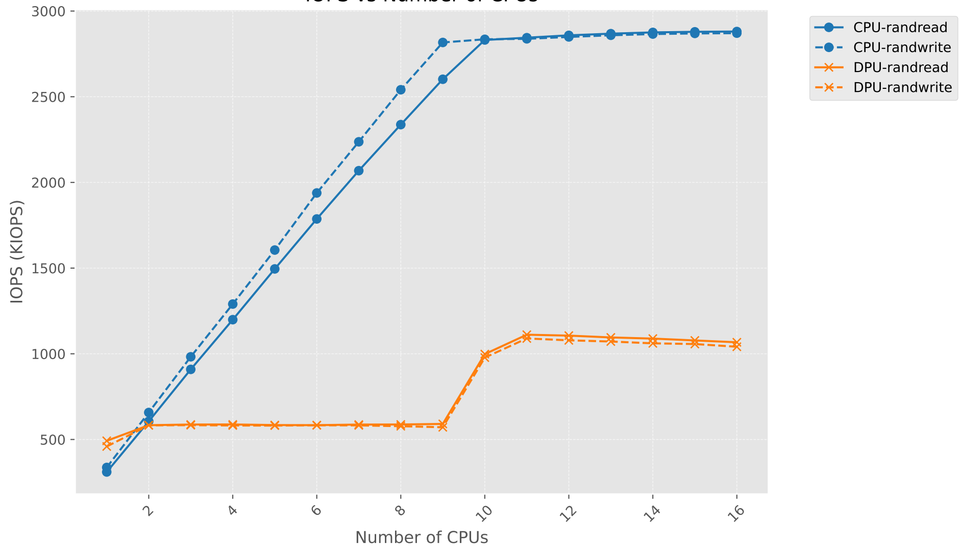
IOPS vs Number of CPUs
